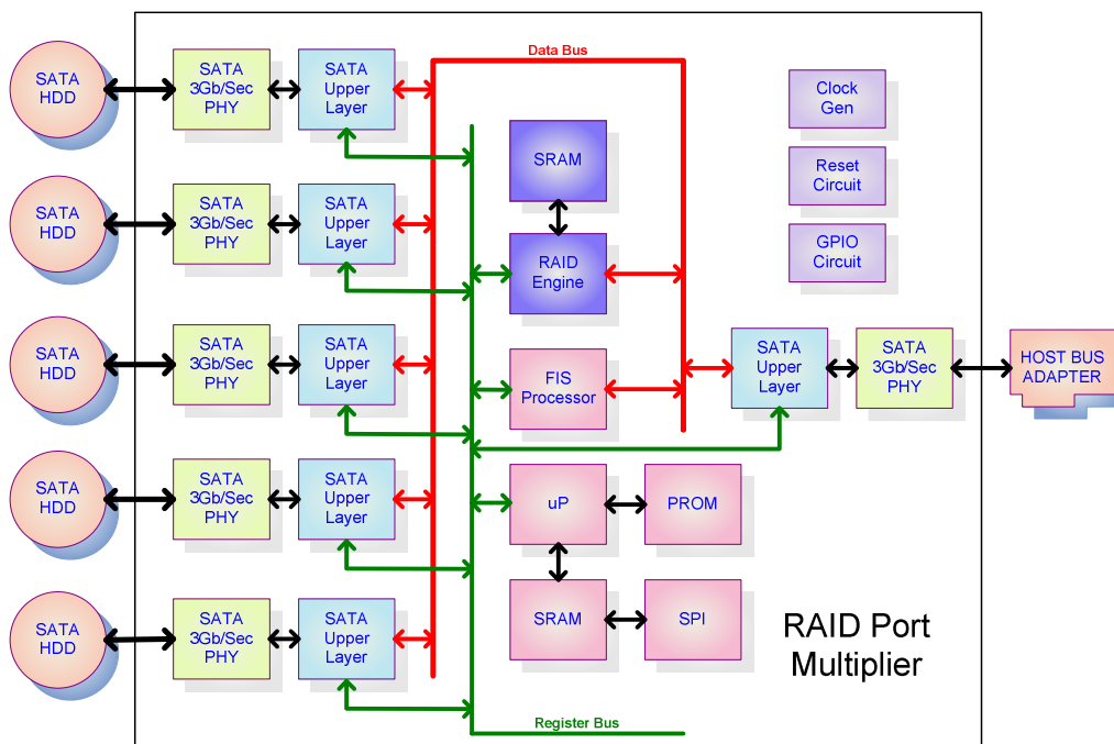
Figure 3.1 Function View of JMB391
