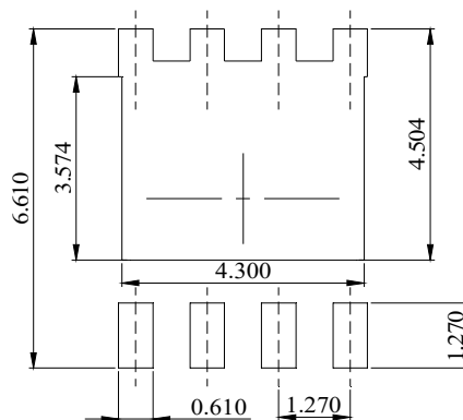
DIMENSIONS: MILLIMETERS
