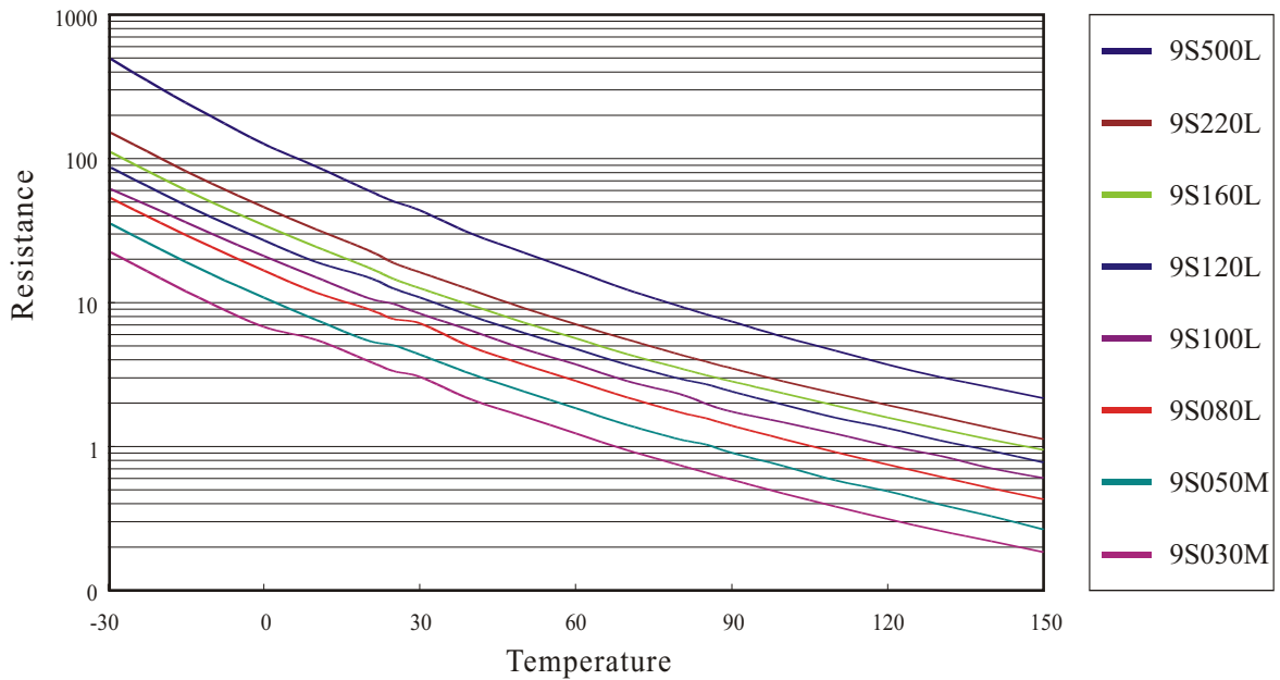
R-T Curve
