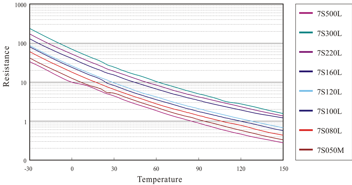
R-T Curve
