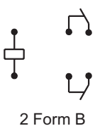
JQX-115F/ □□□□-□□-□-4-□□, 5mm Pinning, 2 Pole, 8A
