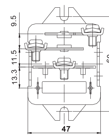
Mounting (Bottom view)
