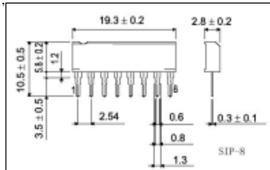
Outline Drawing
