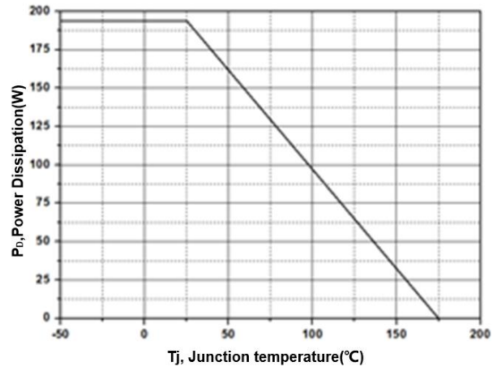
Diode Characteristic
