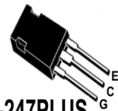
TO-247PLUS
