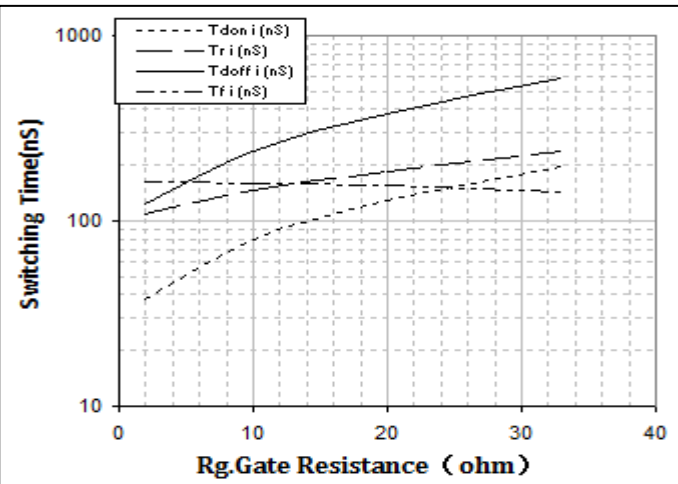
Switching Time vs Rg(25°C) VGE=15V, VCE=600V, IC=75A
