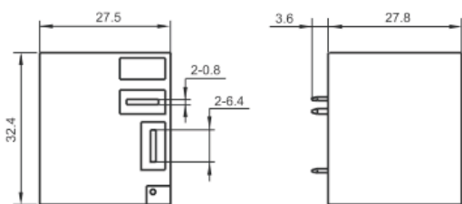
Outline Dimensions
