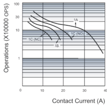
ENDURANCE CURVE
