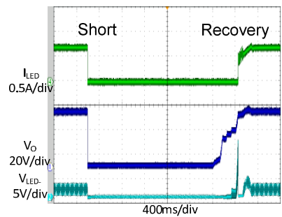
Pre-driver output capacitor short test
