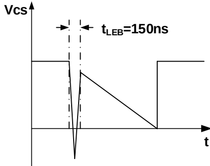
Fig.2 LEB blanking
