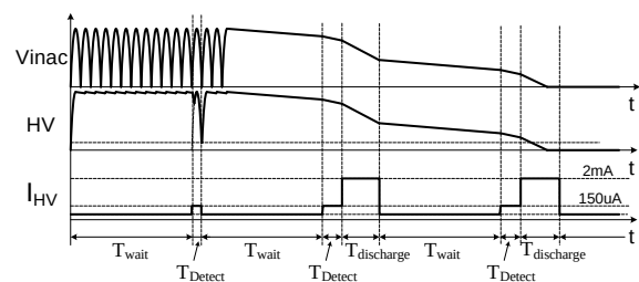
Fig.3 X-cap Discharge
