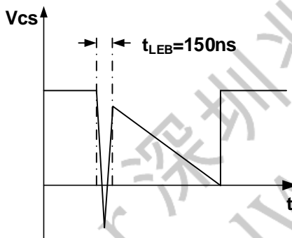
Fig.2 LEB Blanking
