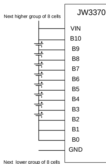
Figure 3. Monitoring 8 Cells with JW3370
