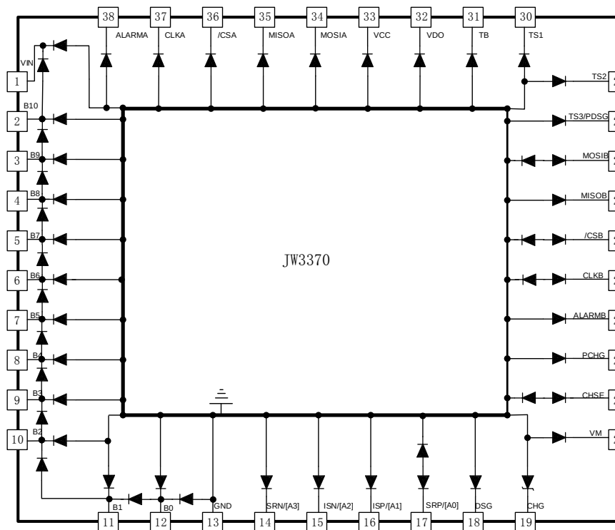
JW3370 Internal ESD Protection Structures
