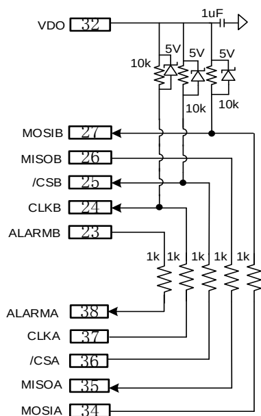
Figure 10. SPI Communication in Cascade Application
