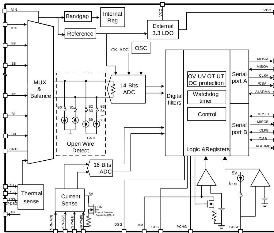
JW3370 Block Diagram
