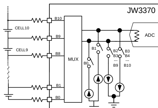
Figure 6. Open Connection
