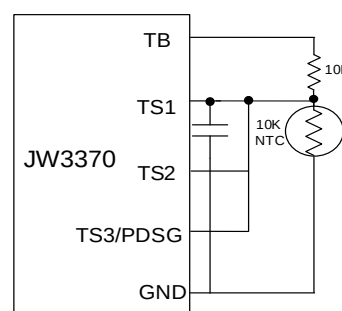
Figure 5. Single channel temperature sensing
