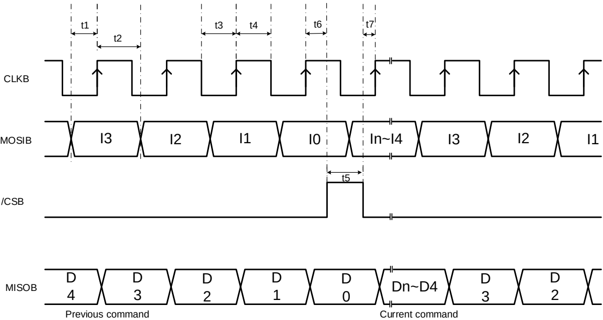
SPI Communication Timing Waveforms
