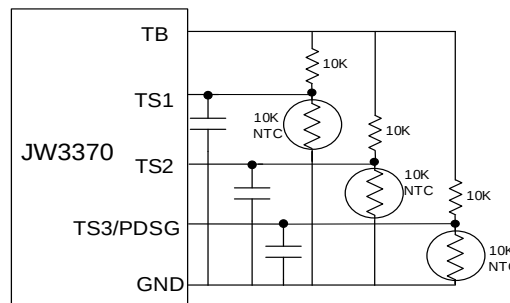
Figure 4. Driving Thermistors Directly from TB
