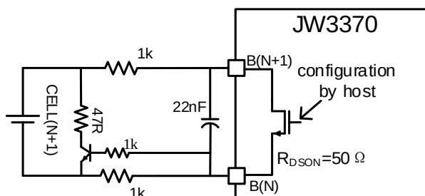
Figure 9. External Discharge Circuit Connection (One cell)
