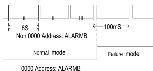
Figure 8. ALARMB State
