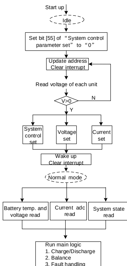
Figure2. Task Handling Flow Chat
