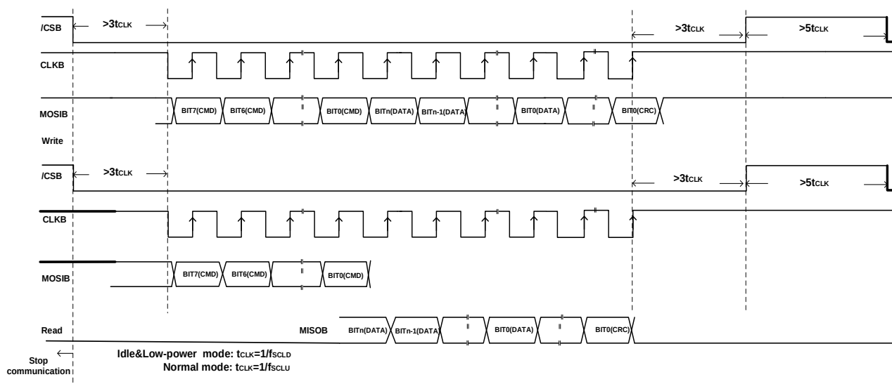
Figure11. Transmission Format
