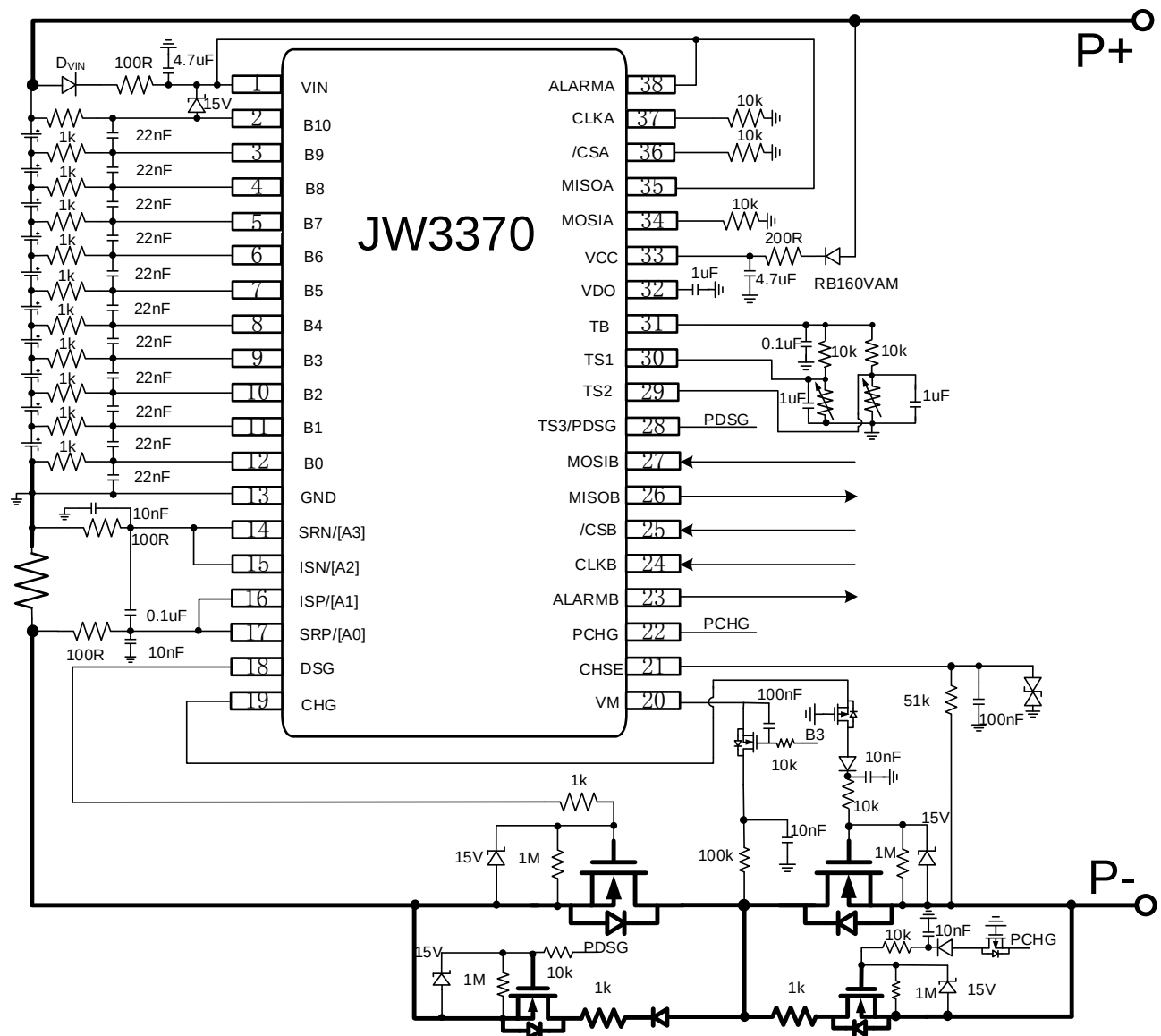
10 Cells Low Side Driver
