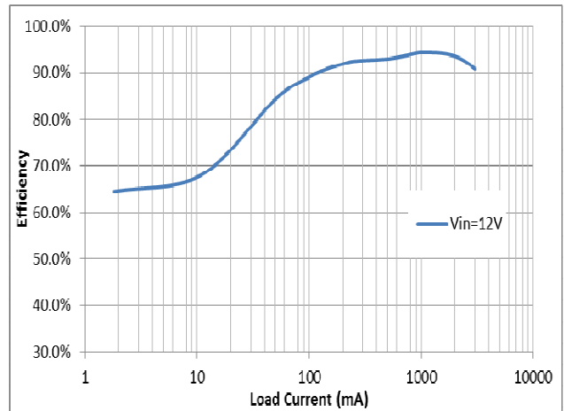
Figure 1. Efficiency vs Load Current (Vout=5V, L=4.7uH)
