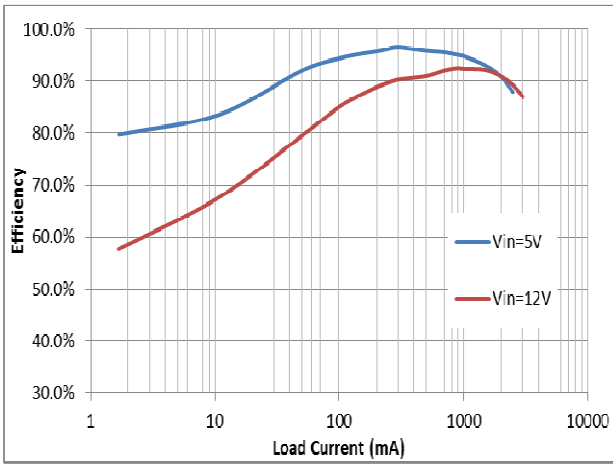
Figure 1. Efficiency vs Load Current (Vout=3.3V, L=4.7uH)
