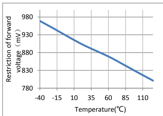
Figure8. Restriction of Forward Voltage vs. Temperature
