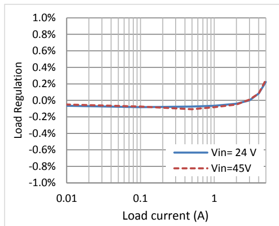
Figure 5. Load Regulation vs Load Current
