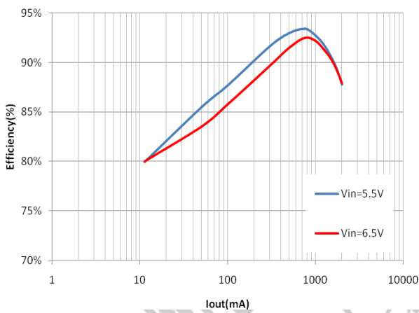
Efficiency @ Vout=1.8V
