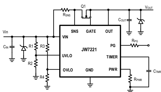
Figure 8. Typical Application
