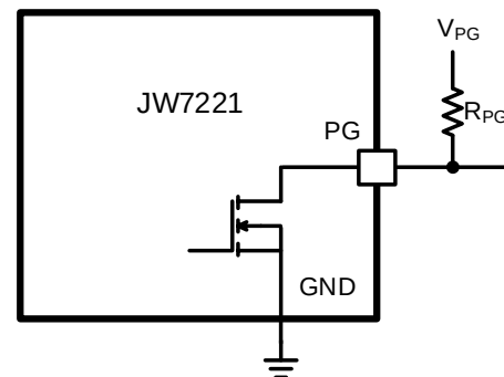
Figure 7. Power Good Output
