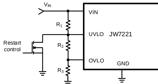
Figure 3. Latched Fault Restart Control
