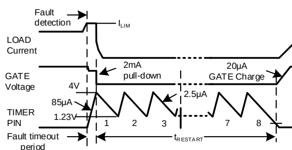
Figure 4. Restart Sequence
