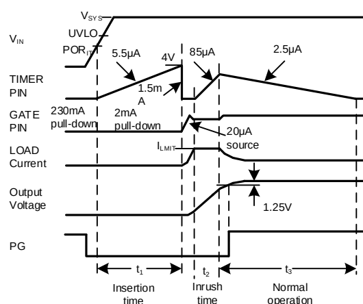
Figure 1. Power-Up Sequence (Current Limit Only)
