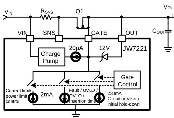
Figure 2. GATE Control
