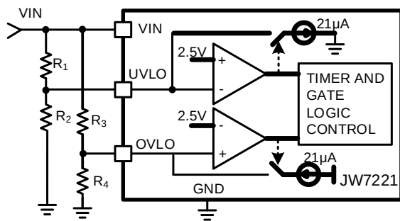
Figure 6. UVLO and OVLO Thresholds Set By R1-R3
