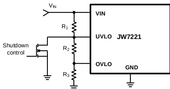
Figure 5. Shutdown Control
