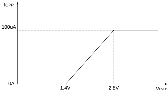
Figure 12 Over power compensation current curve
