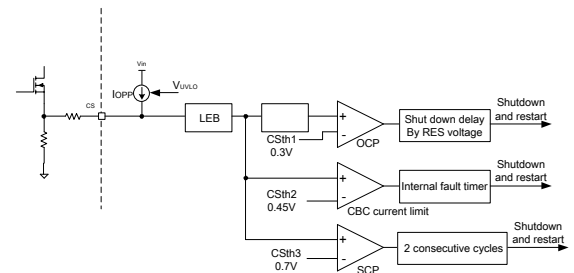
Figure 10. Current sense related protection
