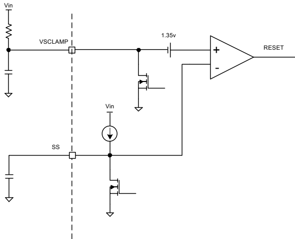
Figure 7. Soft start
