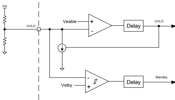
Figure 9. Input under voltage protection
