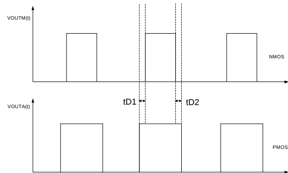
Figure 8. PMOS and NMOS drive overlap
