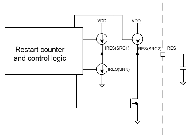
Figure 13. Restart timer
