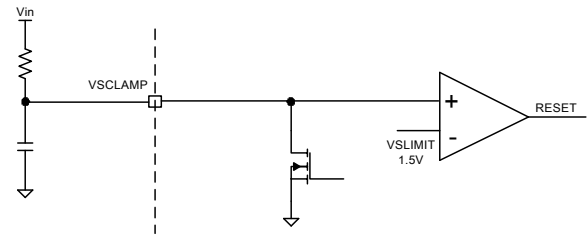
Figure 6. Volt-Second Clamp
