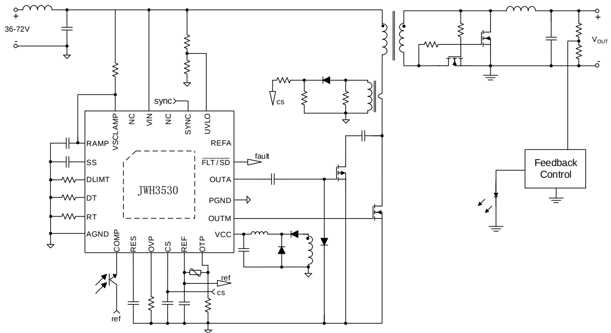
Figure 1. Typical application circuit with voltage mode control
