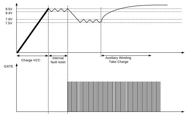
Figure 4. HV start up operation
