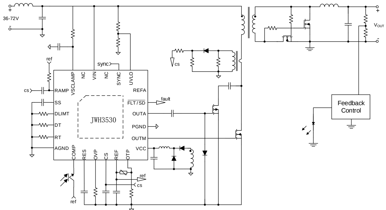
Figure 2. Typical application circuit with current mode control
