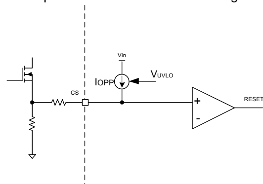
Figure 11. Over power compensation
