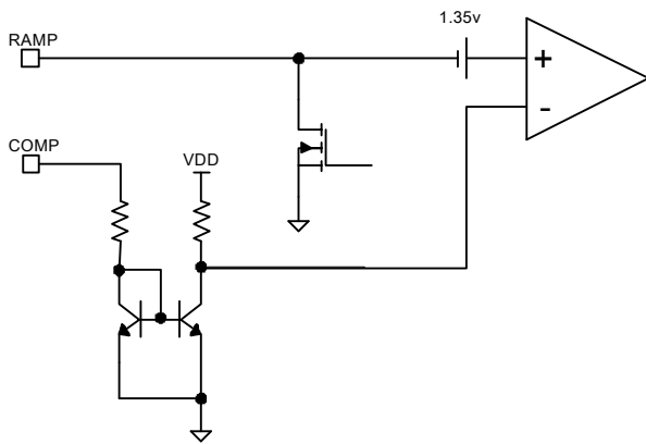
Figure 5. PWM control
