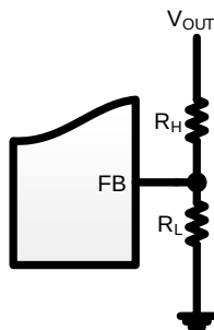
Figure 8. Output Voltage Set
