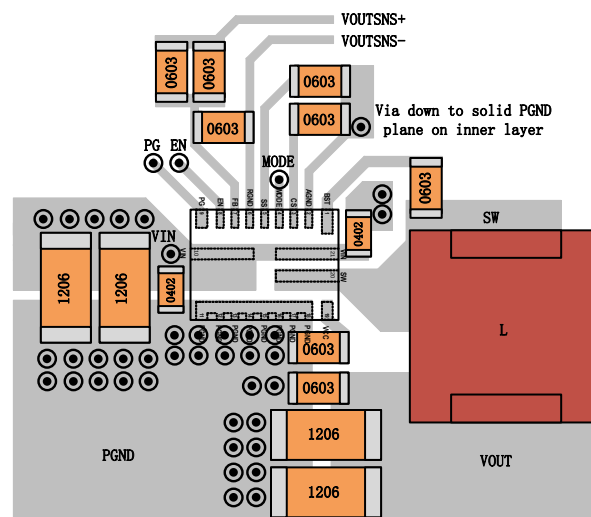
Figure 9. PCB Layout Recommendation
