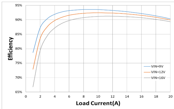
Figure 3. Efficiency vs. Load Current ( V_{OUT}=3.3V , L=0.22\mu H , F_{SW}=1MHz )
