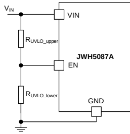
Figure 7. Adjustable UVLO
