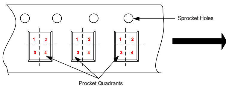
BOTTOM VIEW
