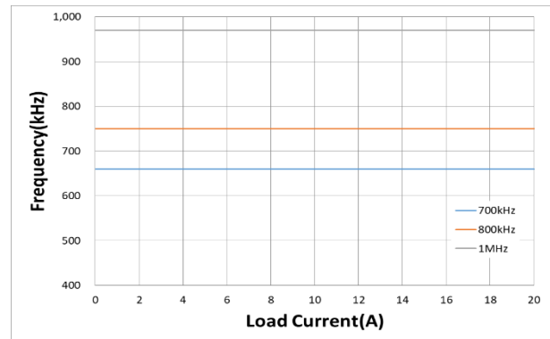
Figure 4. Frequency vs. Load Current ( V_{IN}=12V , V_{OUT}=1.8V , L=0.22\mu H )
