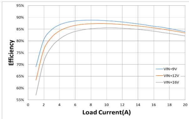
Figure 1. Efficiency vs. Load Current ( V_{OUT}=1.2V , L=0.22\mu H , F_{SW}=700kHz )
