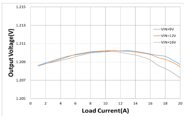
Figure 5. Load Regulation ( V_{OUT}=1.2V , L=0.22\mu H , F_{SW}=700kHz )
