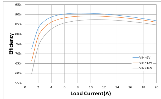
Figure 2. Efficiency vs. Load Current ( V_{OUT}=1.8V , L=0.22\mu H , F_{SW}=1MHz )
