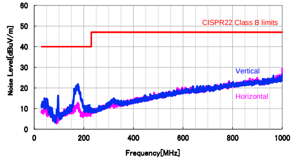
EMI test in CISPR22, Radiated Emission
