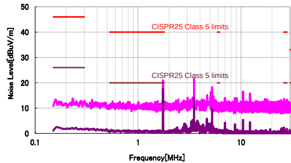
EMI test in CISPR25, Radiated Emission (150k~30M)
