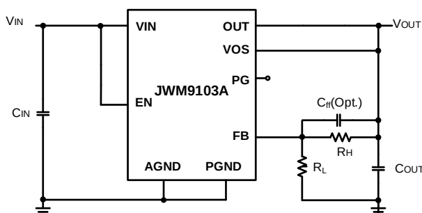
3A Step-down Regulator
