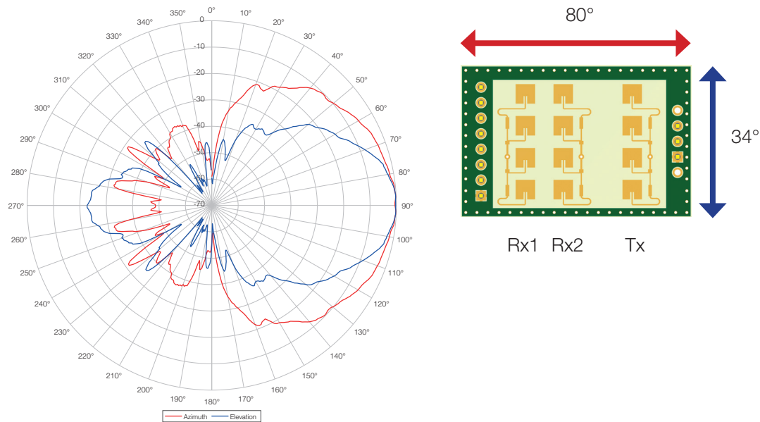
Figure 2: Antenna characteristics
