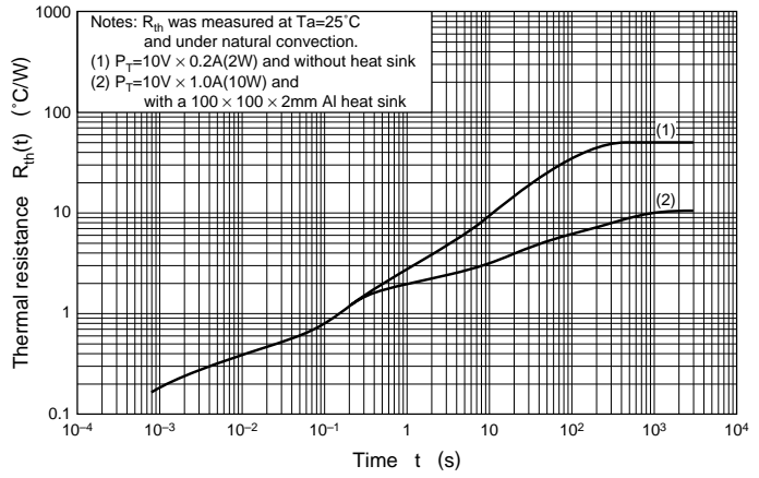
R_{th(t)} - t
