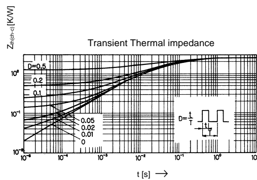
Z_{th(j-c)}
