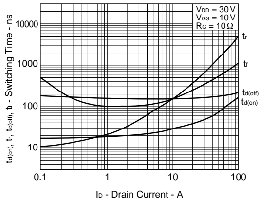
SWITCHING CHARACTERISTICS
