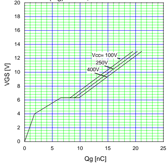
Typical Gate Charge Characteristics V_{GS}=f(Q_g):I_D=3A, T_{ch}=25^\circ C
