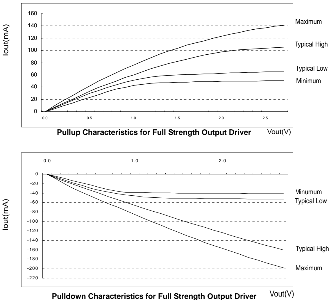
Figure 4. I/V characteristics for input/output buffers: Pull up (above) and pull down (below)
