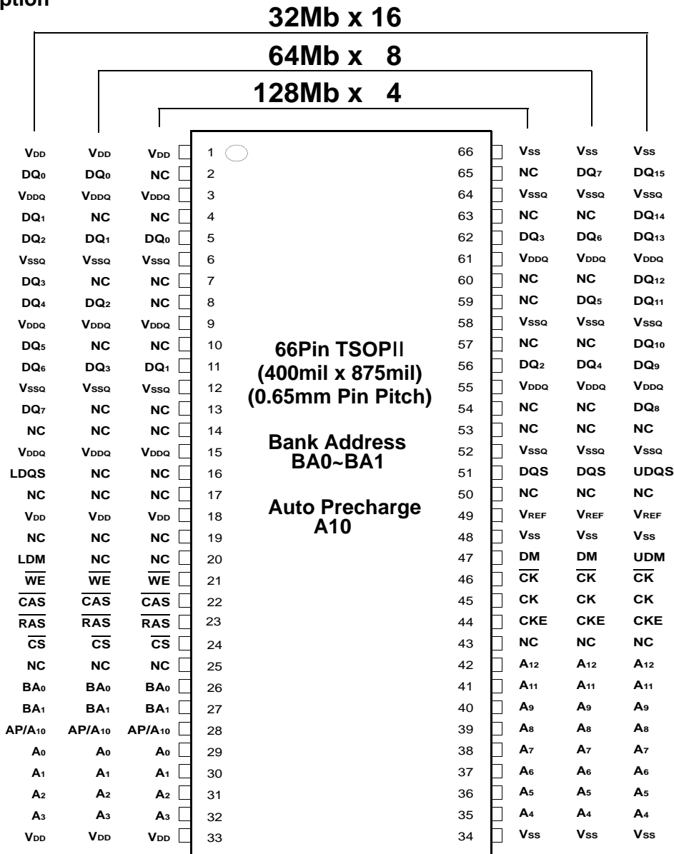
512Mb TSOP-II Package Pinout
