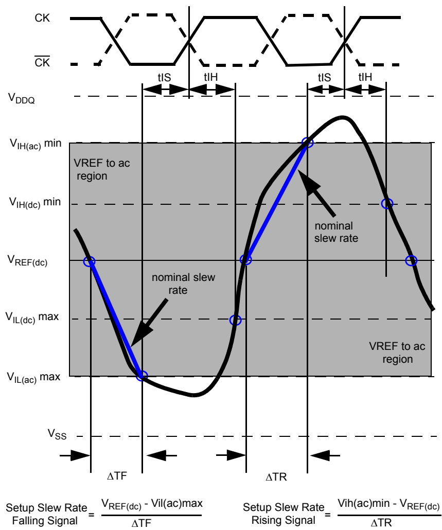
Figure 13 - Illustration of nominal slew rate for tIS
