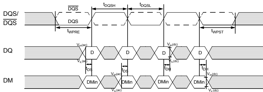
&lt;Data input (write) timing&gt;
