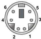
PS/2 Keyboard (6-pin Female)
