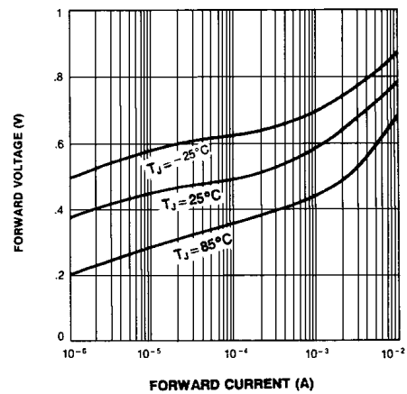
Fig. 4 FORWARD CHARACTERISTICS
