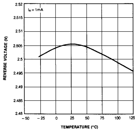
Fig. 3 TEMPERATURE DRIFT
