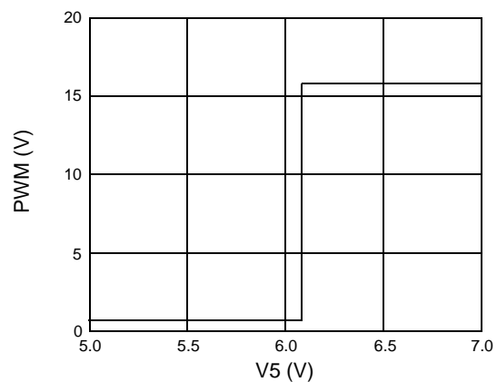
Figure 4. OCP Offset Voltage for 3.3V
