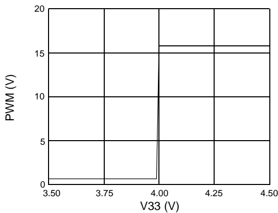
Figure 3. Over Voltage Protection for +3.3V
