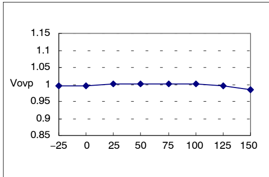
Figure 24. Over Voltage Protection
