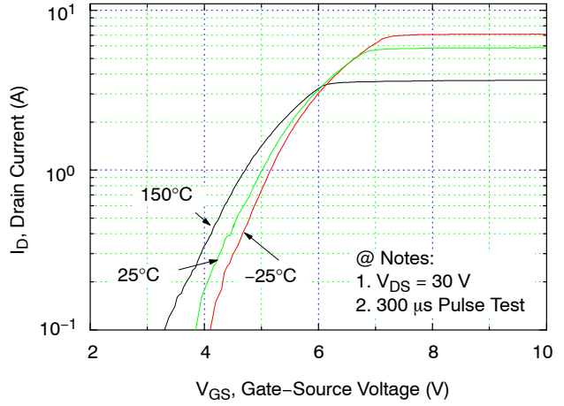
Figure 3. Transfer Characteristics
