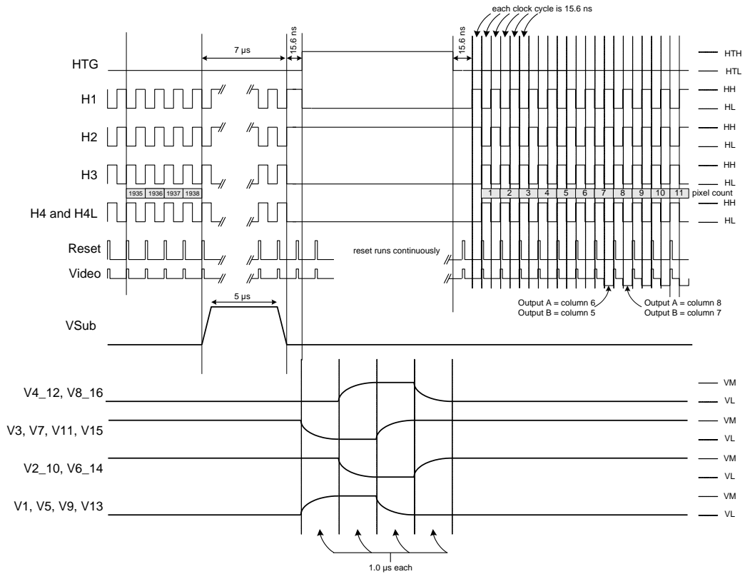
Figure 27: FB2/FB4 Mode –Vertical Timing Sequence - VG
