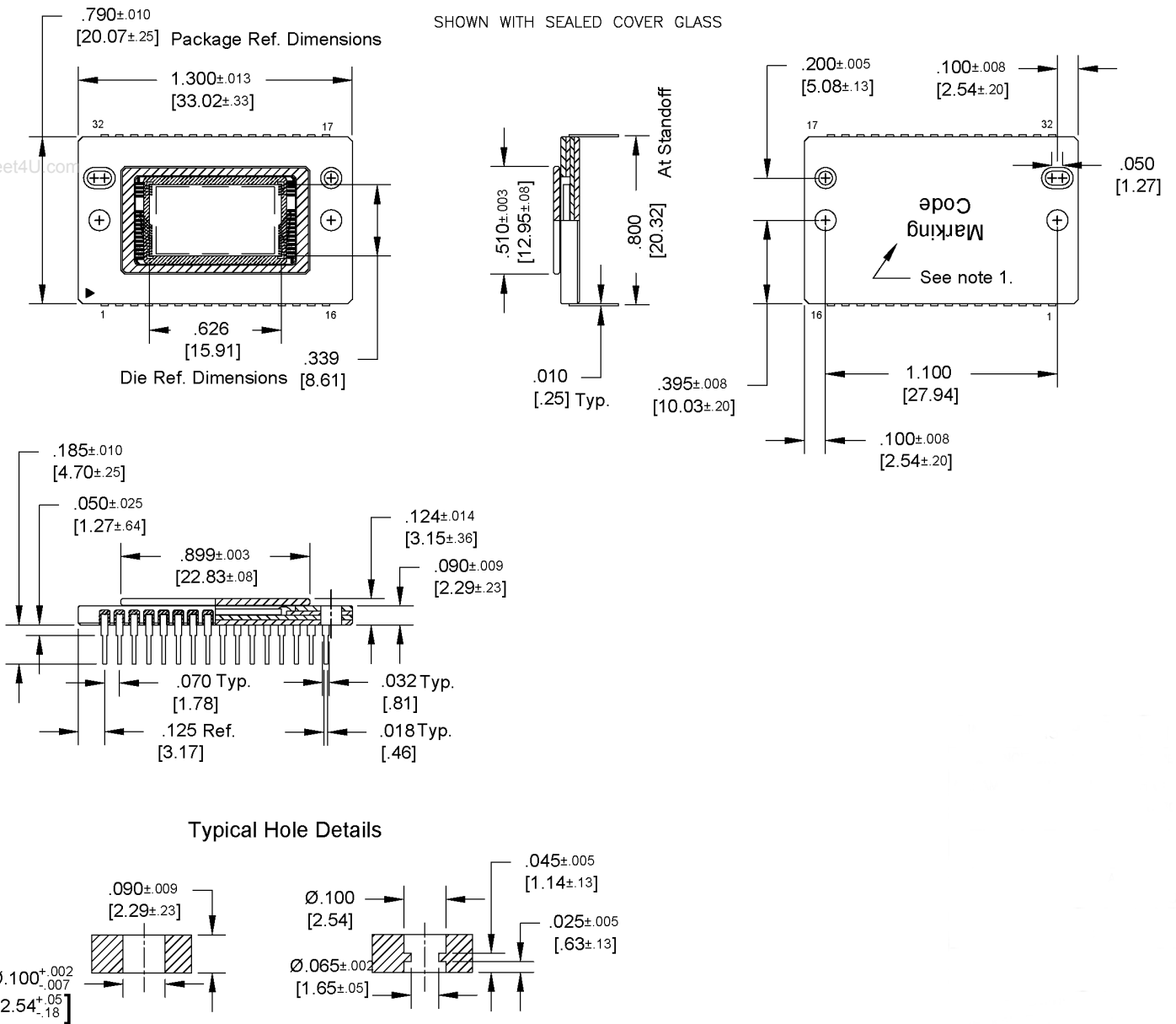
Figure 15: Completed Assembly (1 of 2)
