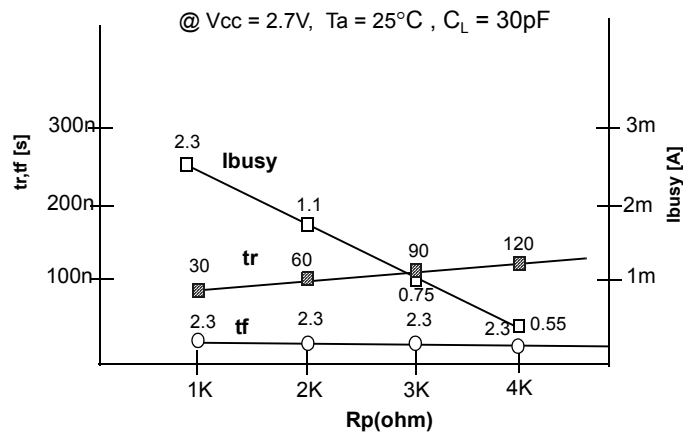
Fig 21 R_p vs t_r, t_f & R_p vs i_{\text{busy}}
