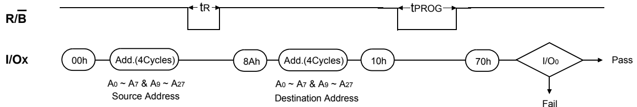
Figure 16. 1-page Copy-Back program Operation
