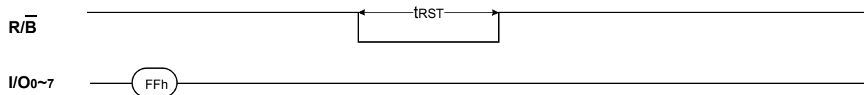
Figure 20. RESET Operation
