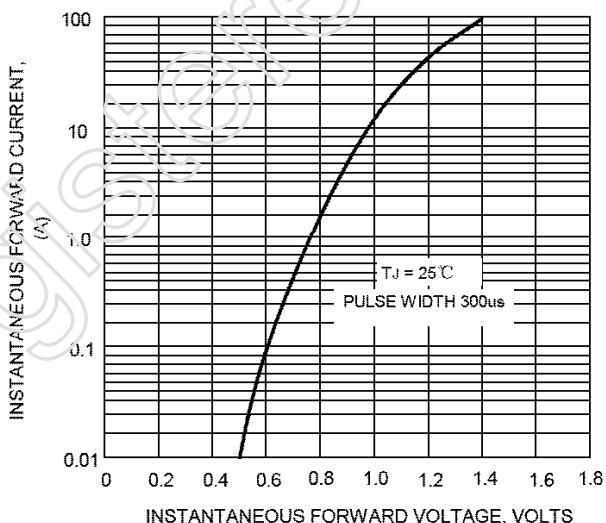
FIG.4-TYPICAL FORWARD CHARACTERISTICS
