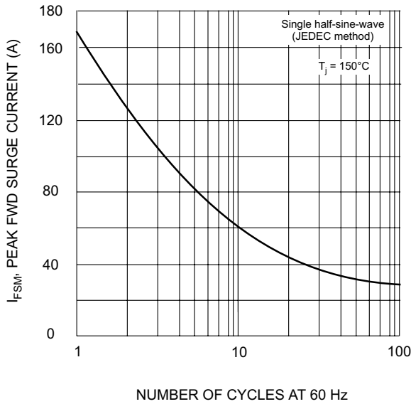
NUMBER OF CYCLES AT 60 Hz Fig. 3 Max Non-Repetitive Surge Current
