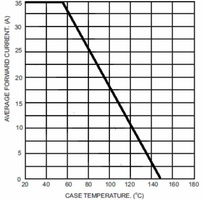
FIG.2- MAXIMUM FORWARD CURRENT DERATING CURVE
