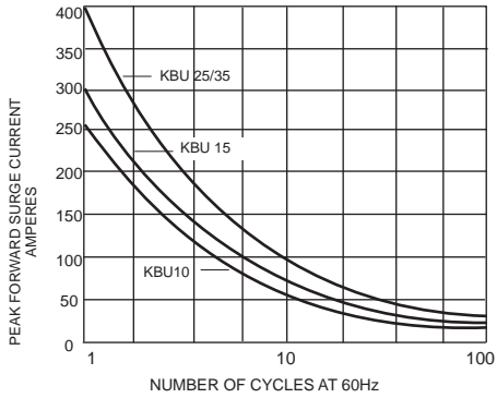
FIG.1 -MAXIMUN FORWARD SURGE CURRENT
