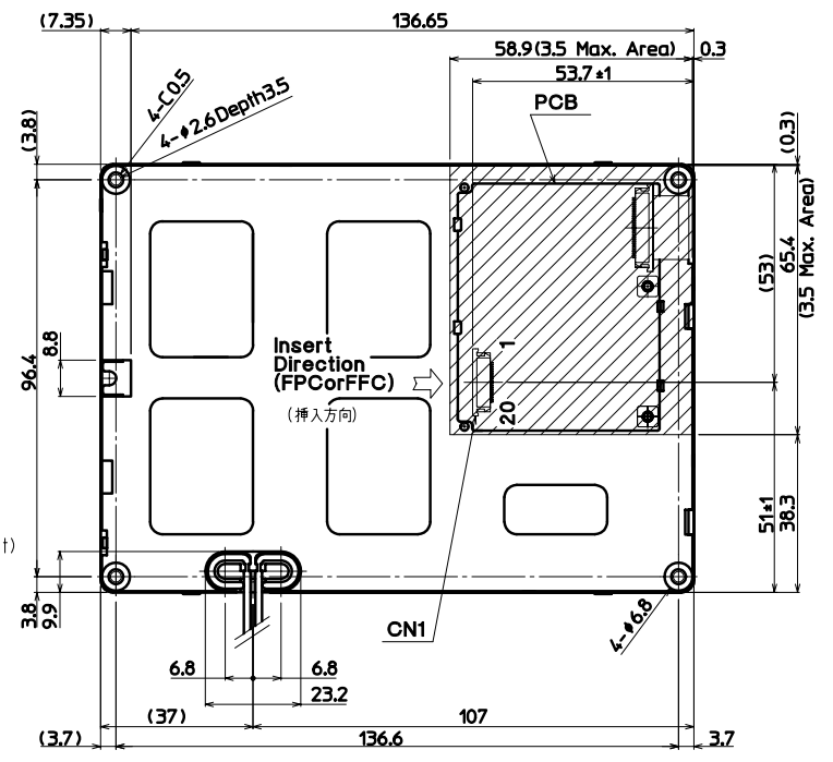
△ Back side drawing (1:2)
