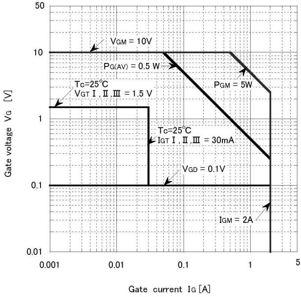
Gate characteristic
