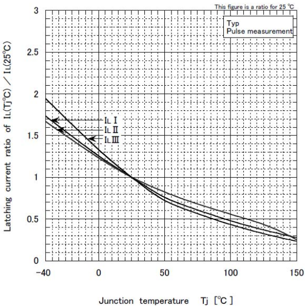
Latching current ratio vs Junction temperature
