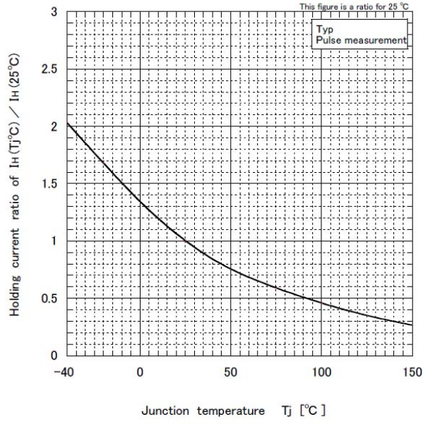
Holding current ratio vs Junction temperature
