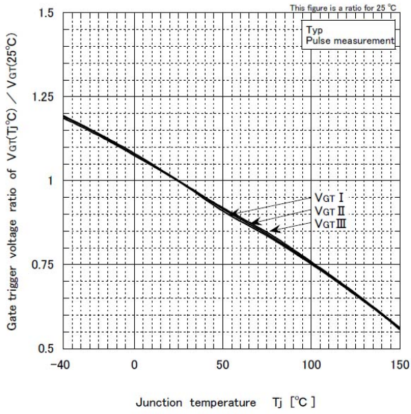
Gate trigger voltage ratio vs Junction temperature
