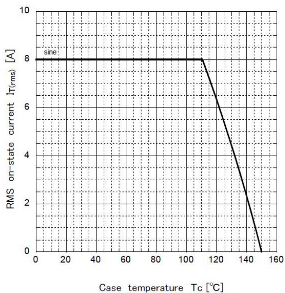
Derating curve T_c - I_{T(rms)}
