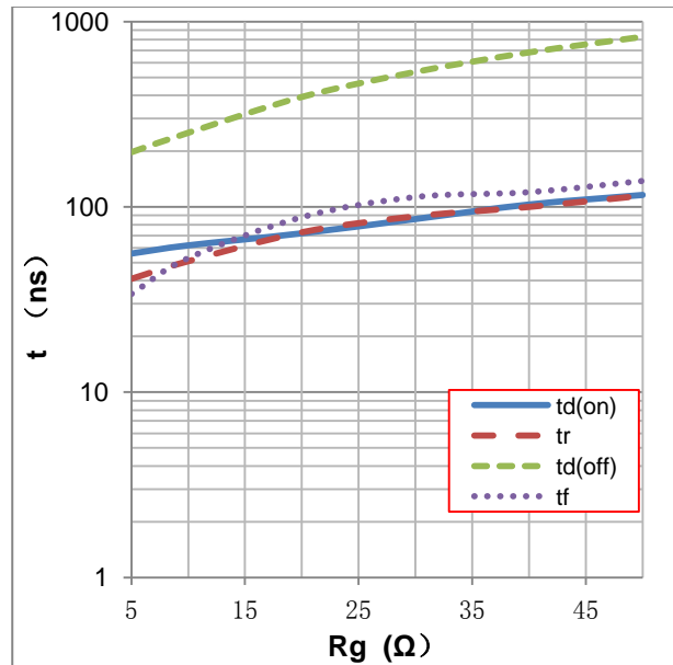
Figure12: typical switching time VS. Rg, TC=25°C, L=500uH, VCE=300V, VGE=15V, IC=50A
