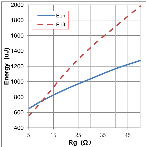
Figure11: typical energy loss VS. Rg, TC=25°C, L=500uH, VCE=300V, VGE=15V, IC=50A
