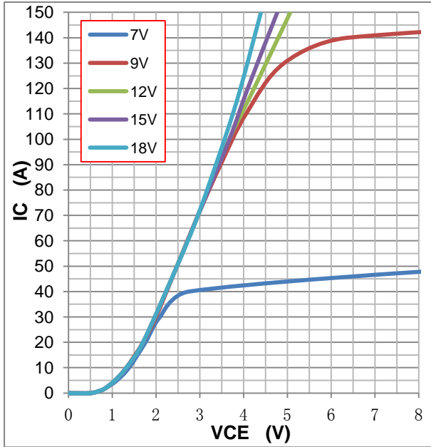
Figure5: typical IGBT output characteristics, T_J=25^{\circ}\text{C}; t_p=300\mu\text{s}
