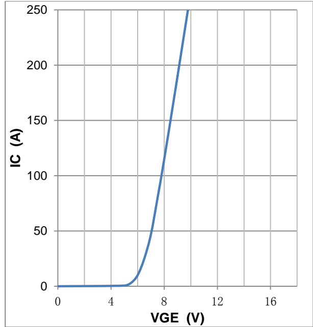
Figure6: typical trans characteristics, V_{CE}=20\text{V}, t_p=20\mu\text{s}
