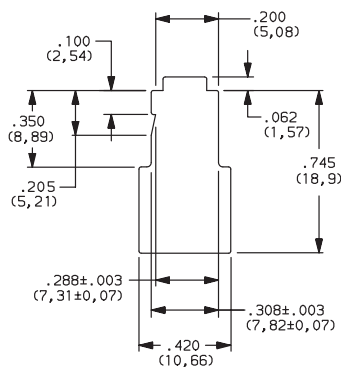
PANEL CUT-OUT (THICKNESS .040)
