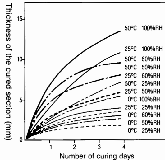
Relationship between the curing speed and the temperature
