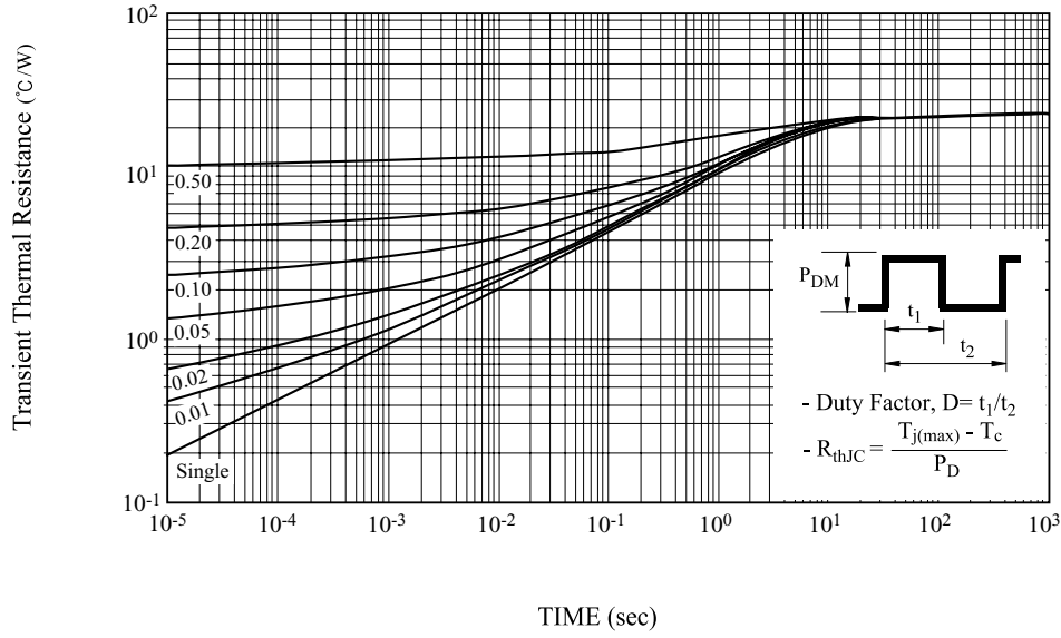
Fig11. Transient Thermal Response Curve [ R_{thJC} ]
