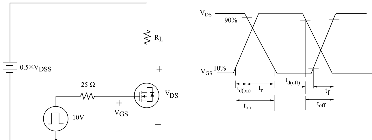
Fig15. Resistive Load Switching
