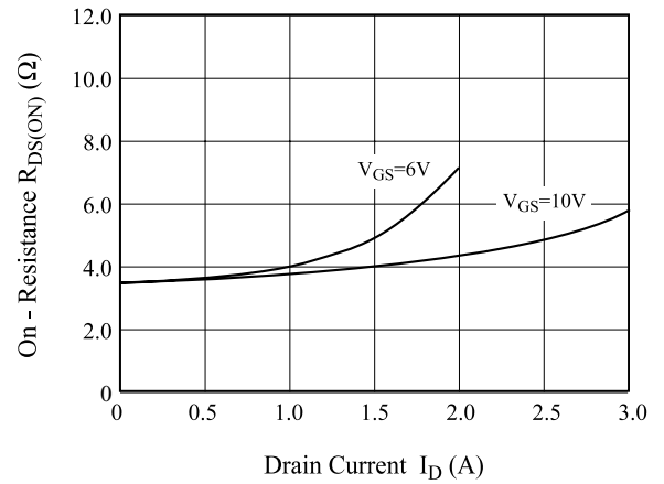
Fig4. R_{DS(ON)} - I_D
