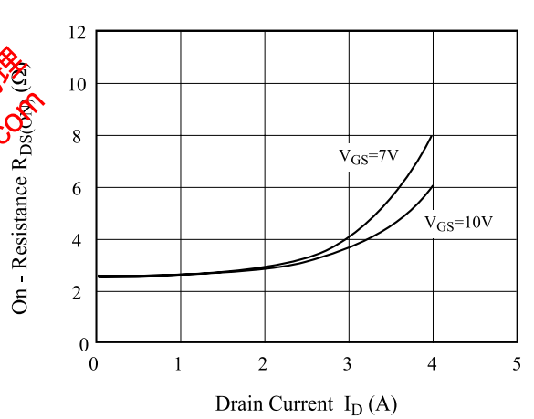
Fig4. R_{DS(ON)} - I_D
